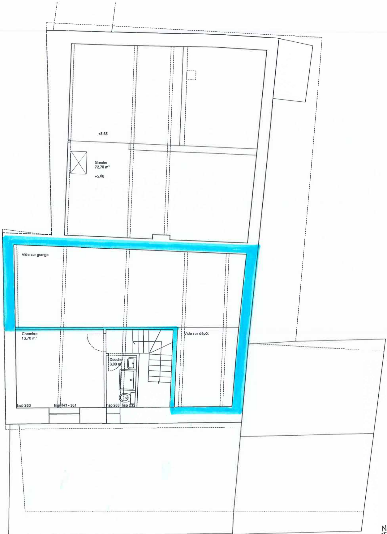
PLAN COMBLE
